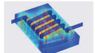
Microcoil with integrated soft magnetic core
