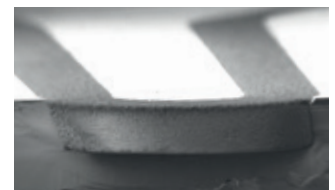
Cross section of a porous microfluidic structure
